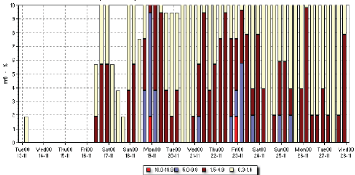
Example – Precipitation (rrr6) – EPS-run: 2018-11-13 00:00
