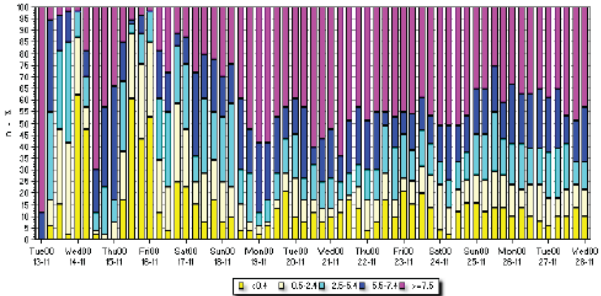
Example – Clouds (n) – EPS-run: 2018-11-13 00:00
