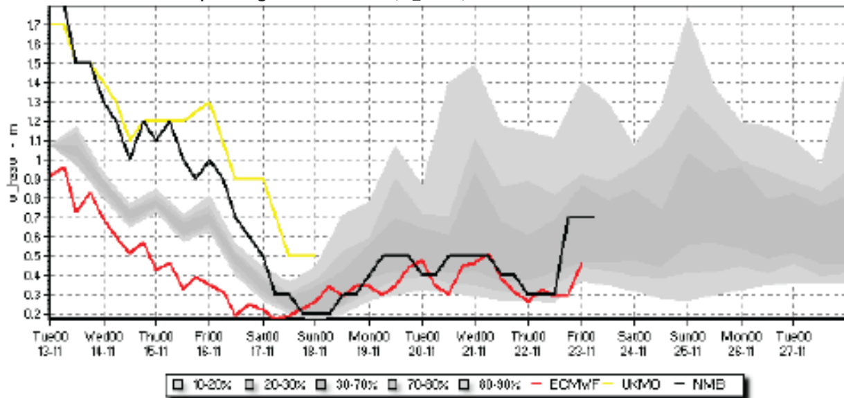
Example – Significant Waves (w_hssw) – EPS-run: 2018-11-13 00:00
