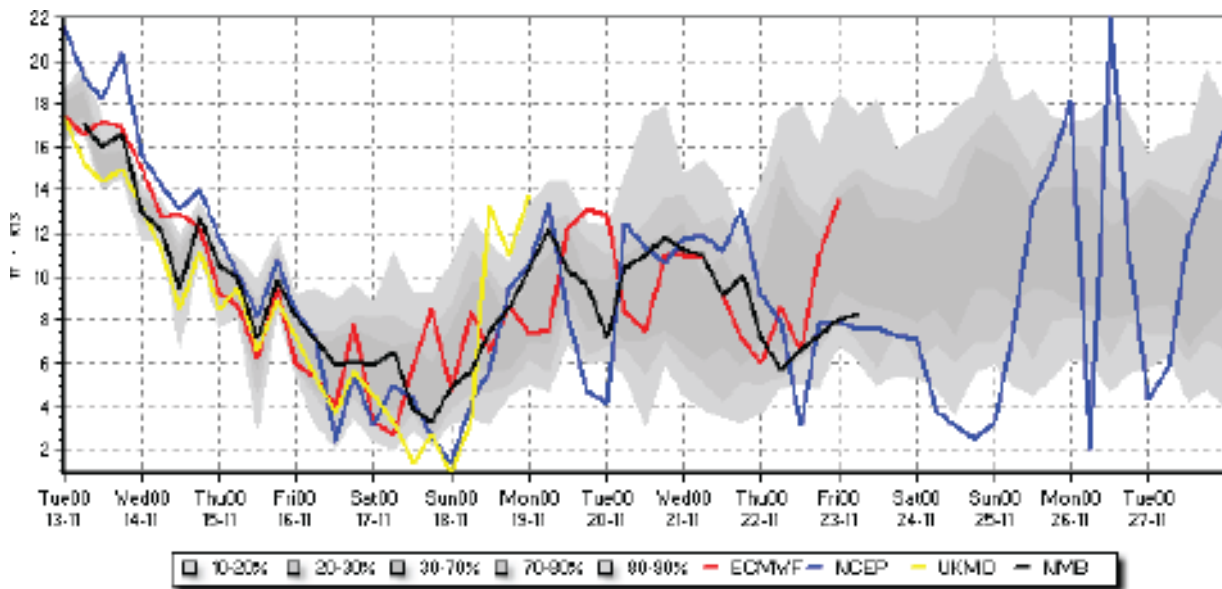
Example – Wind speed (ff) – EPS-run: 2018-11-13 00:00
