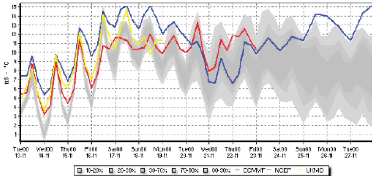
Example - Temperature (tt6) - EPS-run: 2018-11-13 00:00
